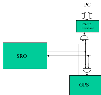
Figure 2 - Communication Diagram (Switch S6 to the left)
