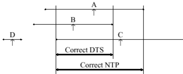
Figure 16. Confidence Intervals and Intersections
