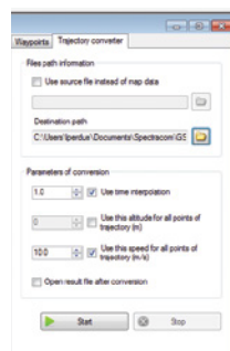
Figure 4: Trajectory Converter
