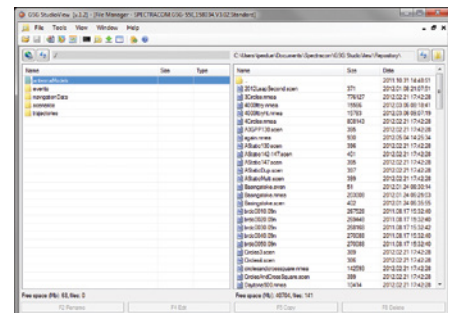
Figure 7: File Manager
